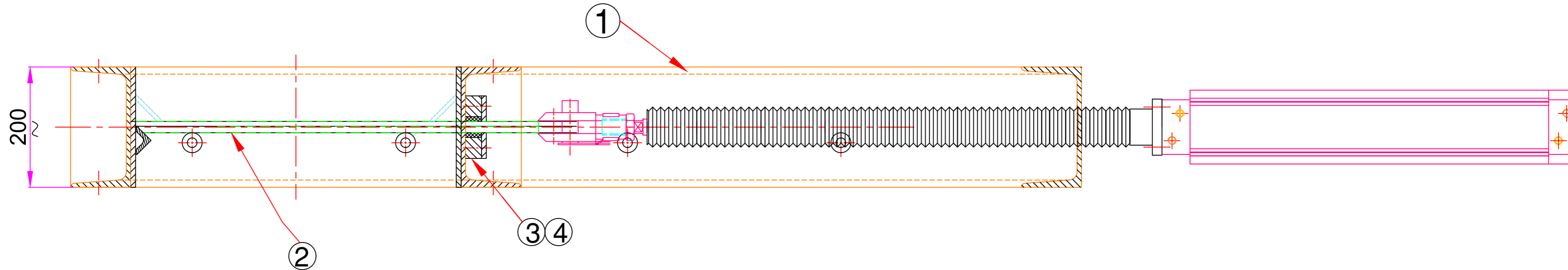
SECTION X-X
